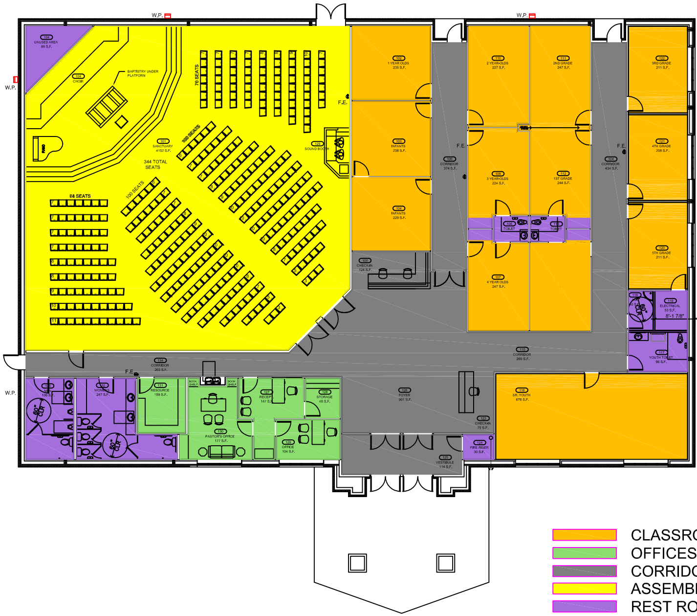
FLOOR PLAN
